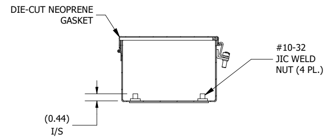
SECTION L-L VIEW (INSIDE TOP OF ENCL.)
