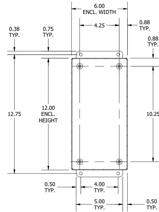
SECTION K-K (INSIDE BACK OF ENCLOSURE)
