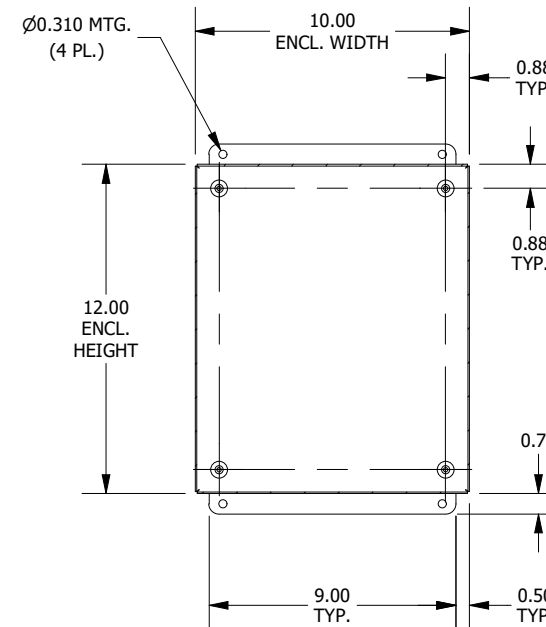
SECTION K-K (INSIDE BACK OF ENCLOSURE)
