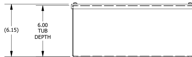
BOTTOM VIEW
