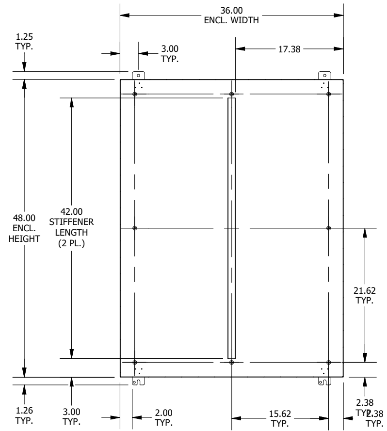
SECTION C-C (INSIDE BACK OF ENCLOSURE)
