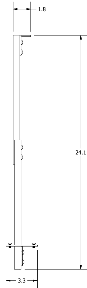
ASSM. FRONT VIEW
