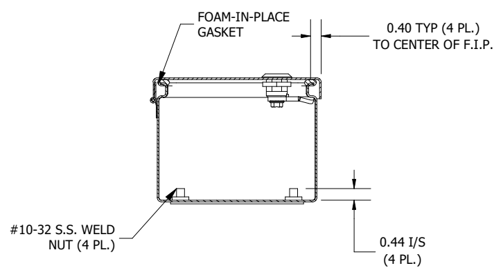
SECTION A-A (INSIDE TOP OF ENCL.)
