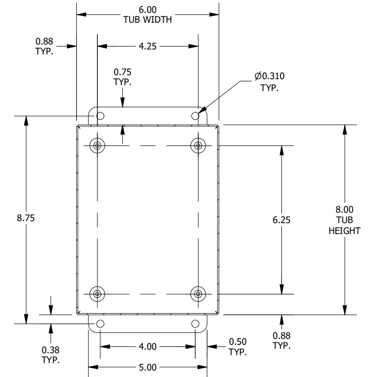
SECTION K-K VIEW (INSIDE BACK OF ENCL.)
