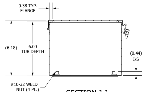
SECTION J-J (INSIDE TOP OF ENCL.)
