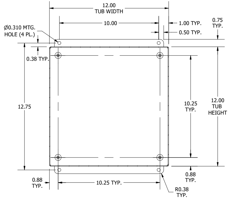
SECTION F-F (INSIDE BACK OF ENCL.)
