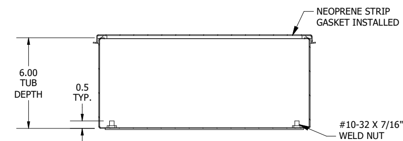
SECTION L-L VIEW (INSIDE TOP OF ENCL.)
