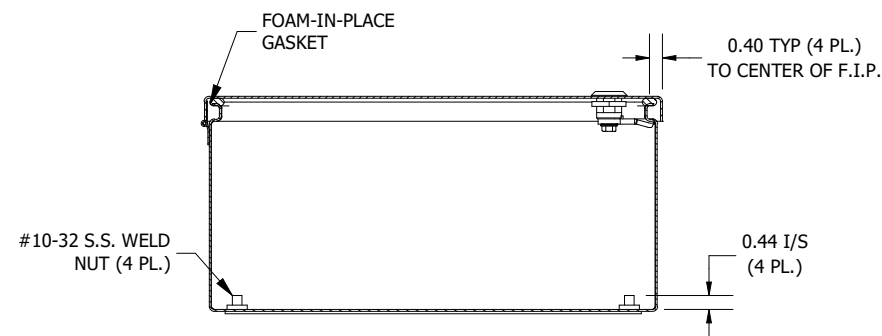
SECTION A-A (INSIDE TOP OF ENCL.)
