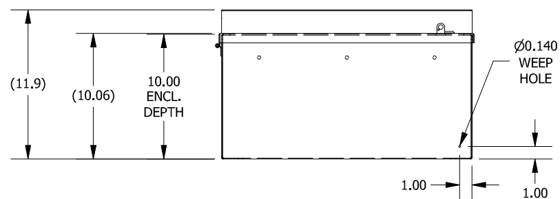
BOTTOM VIEW
