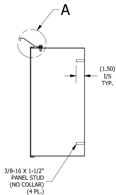
SECTION B-B (INSIDE LEFT OF ENCL.)
