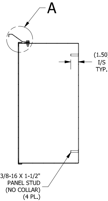
SECTION B-B (INSIDE LEFT OF ENCL.)
