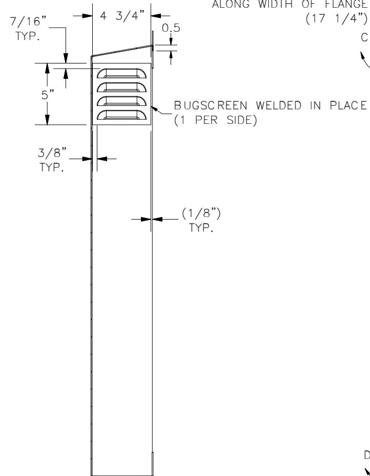
SECTION A-A VIEW (INSIDE LEFT OF HOOD)
