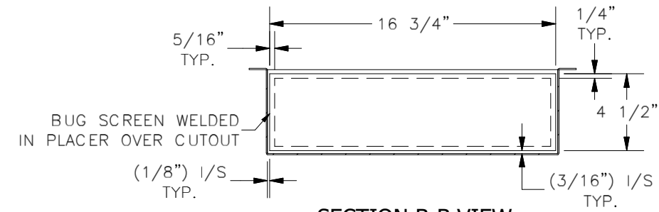
SECTION B-B VIEW (INSIDE BOTTOM OF HOOD)
