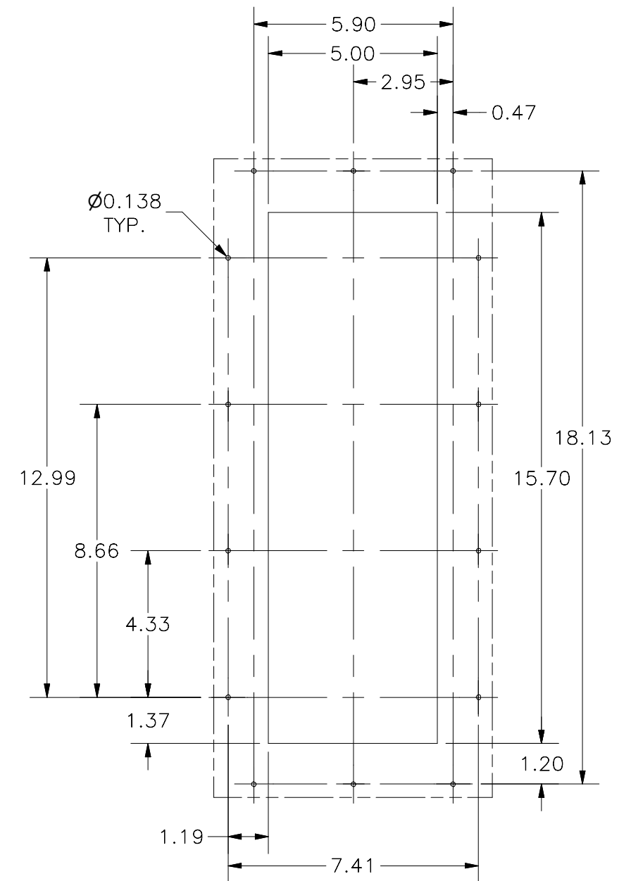
DETAIL B
