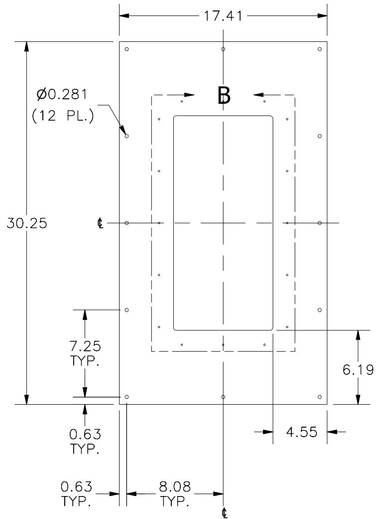
FRONT VIEW (PLATE ONLY)
