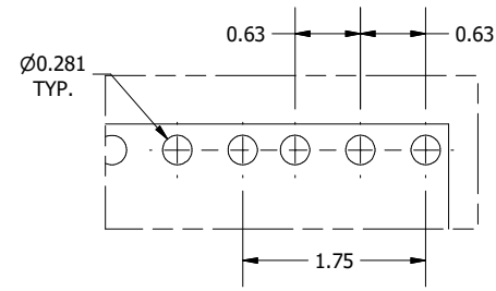
DETAIL A (TYP.) (REPEATING PATTERN FOR STANDARD 19" RACK EQUIPMENT, 16U)
