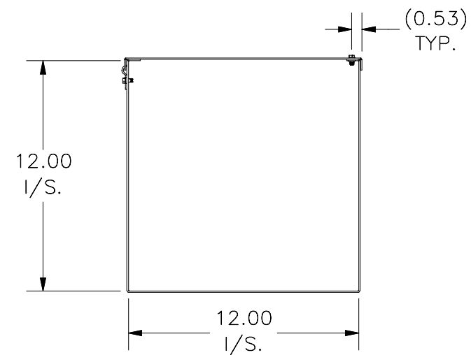
RIGHT VIEW
