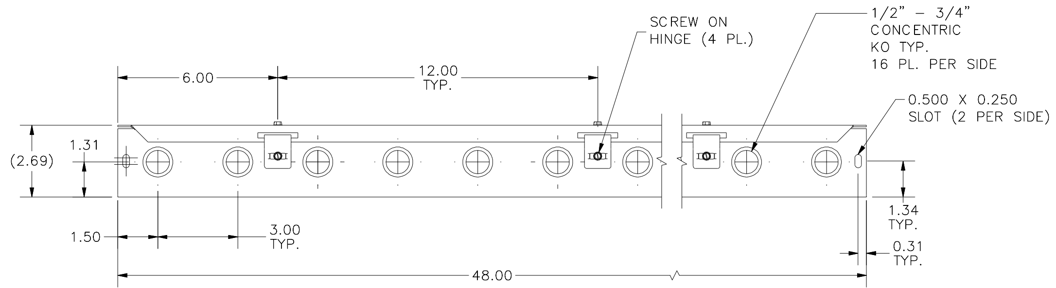
FRONT VIEW
