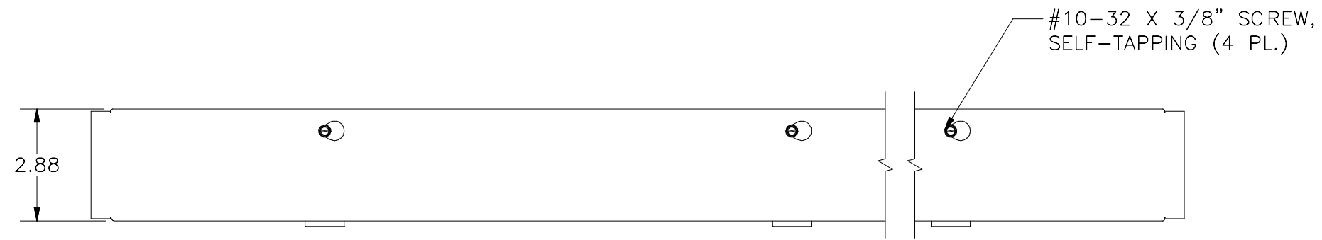
TOP VIEW
