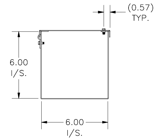
RIGHT VIEW
