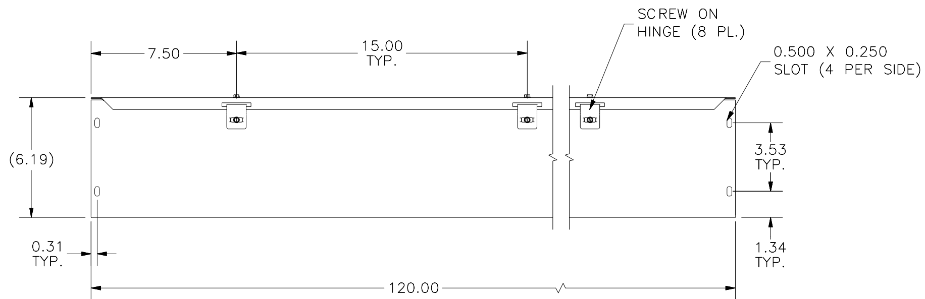
FRONT VIEW
