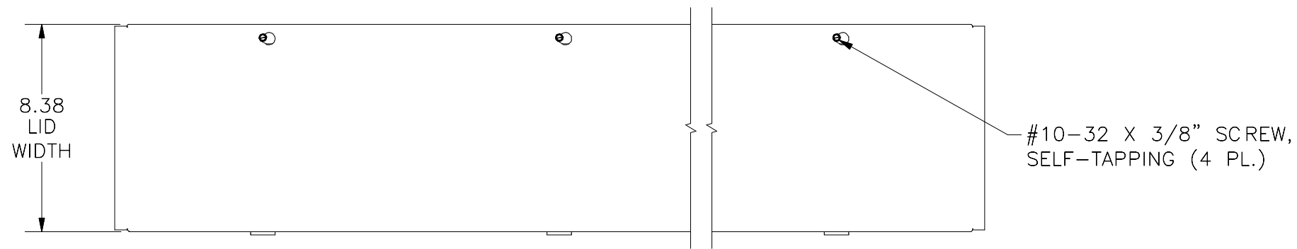
TOP VIEW
