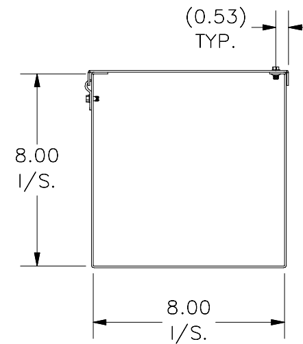
RIGHT VIEW
