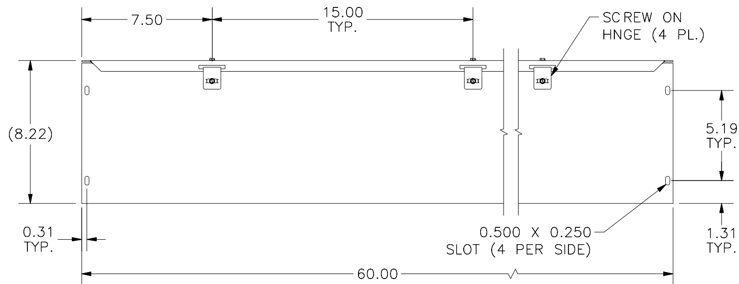
FRONT VIEW
