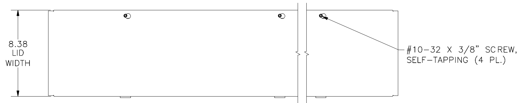
TOP VIEW
