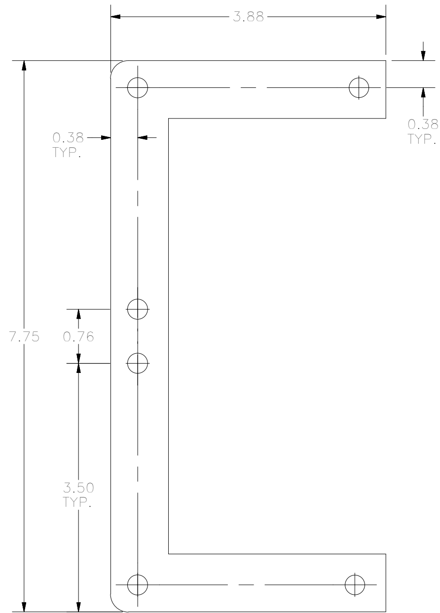
FRONT VIEW
