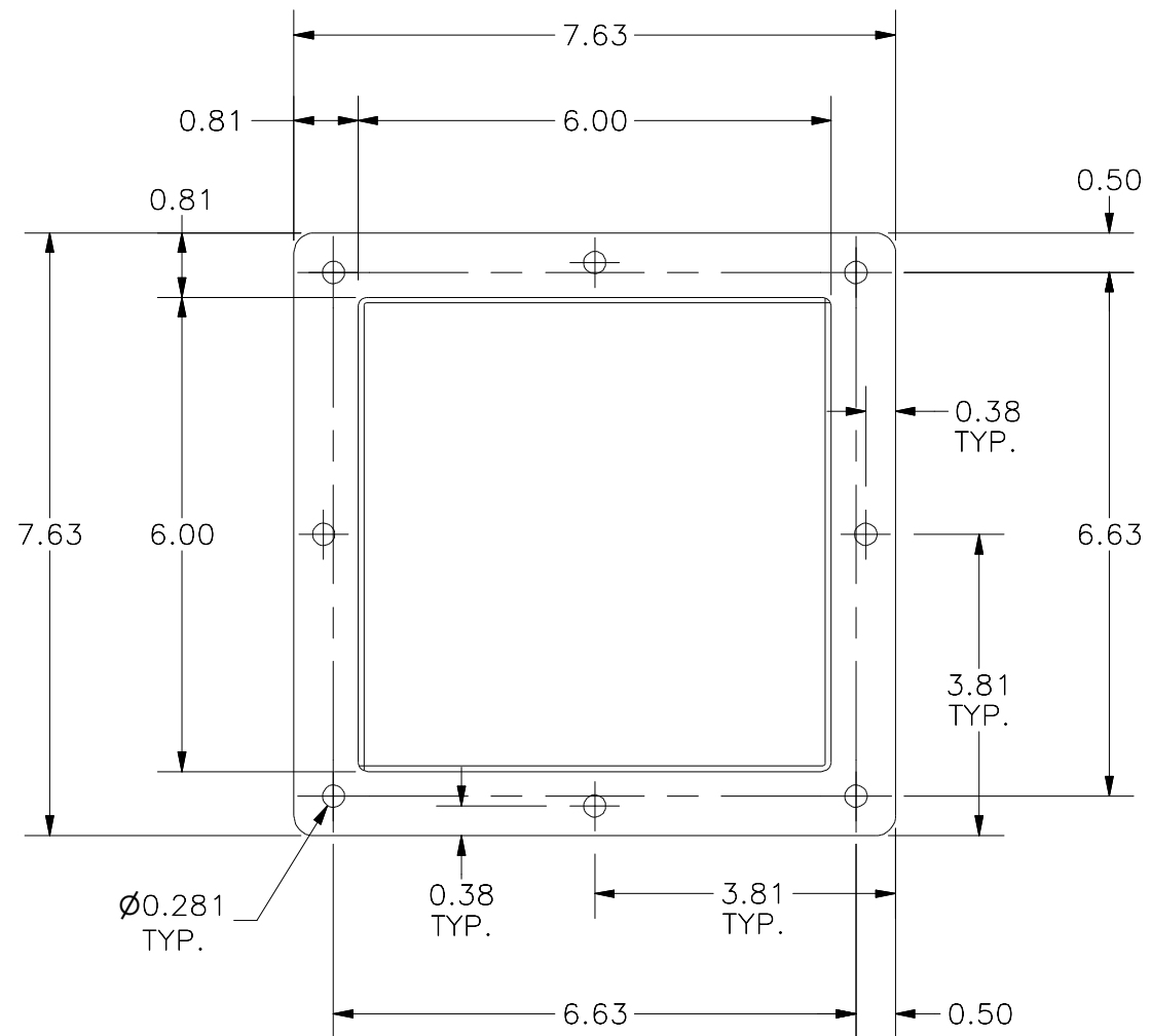
FRONT VIEW
