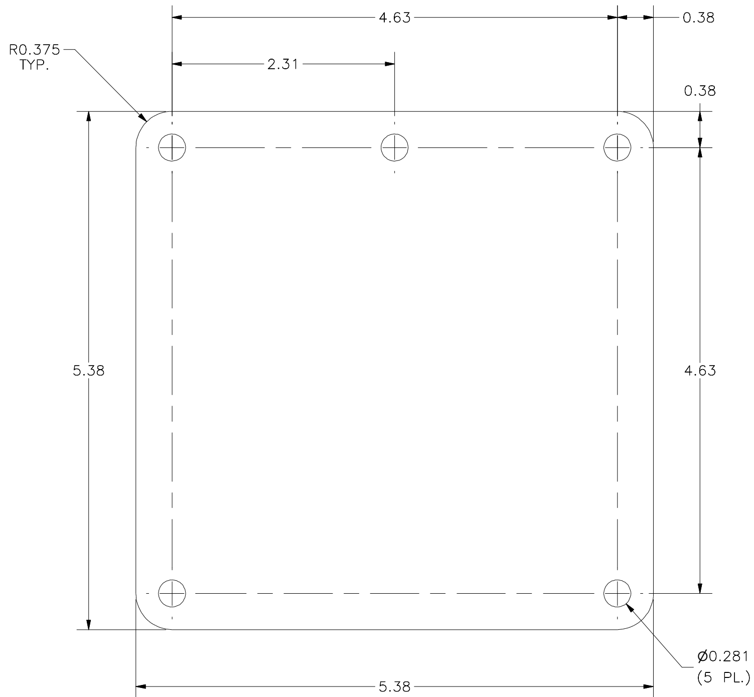
FRONT VIEW
