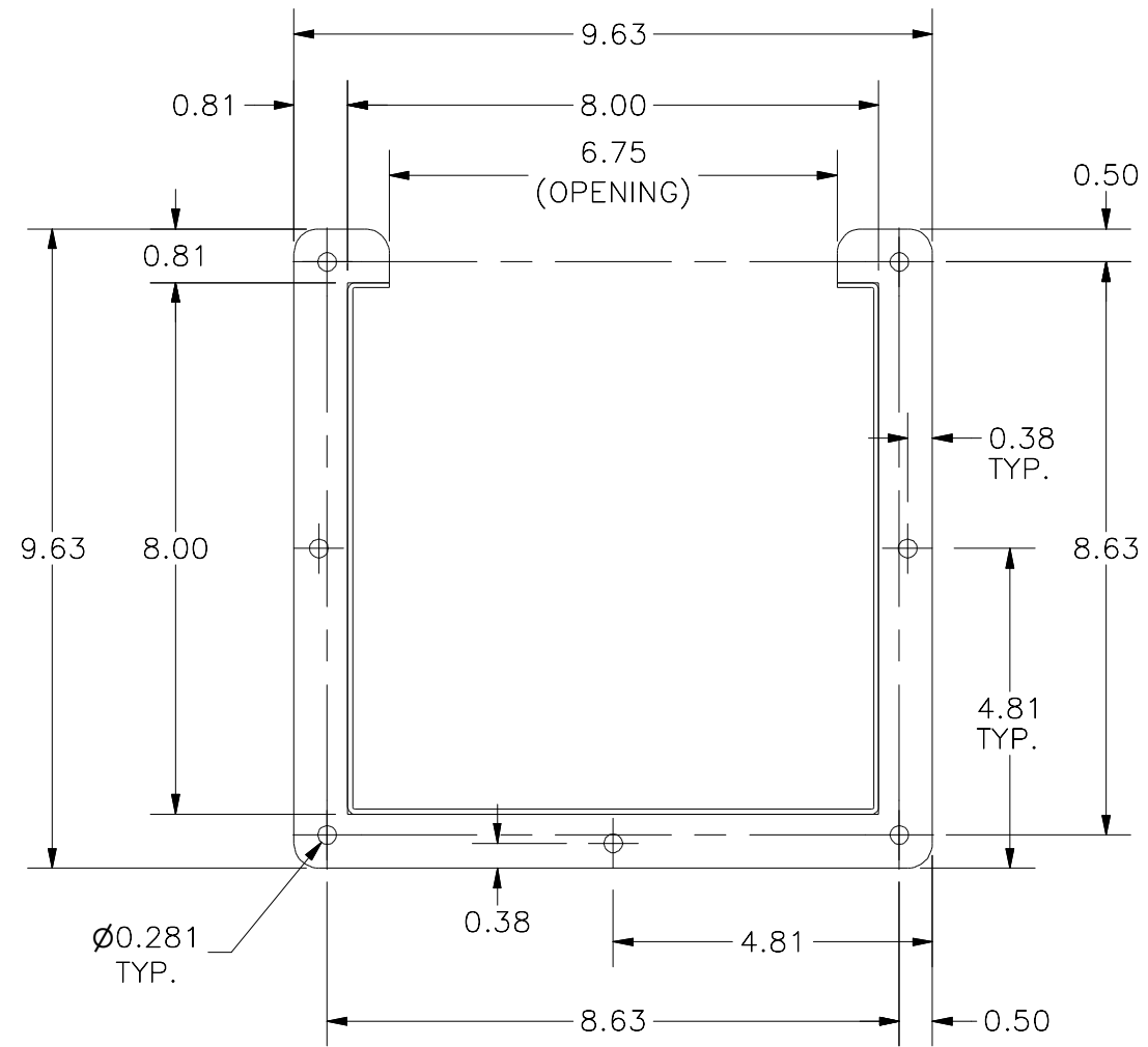
FRONT VIEW
