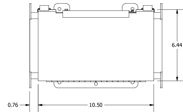
VIEW AC-AC (BACK LID VIEW)
