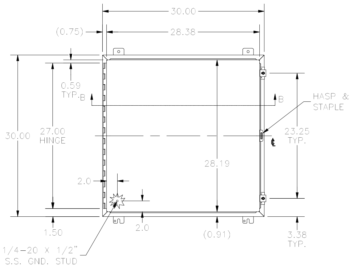
FRONT VIEW
