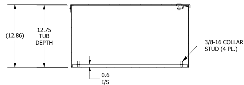
SECTION A-A (INSIDE TOP OF ENCL.)
