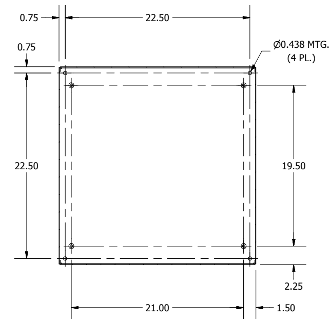
SECTION B-B (INSIDE BACK OF ENCL.)
