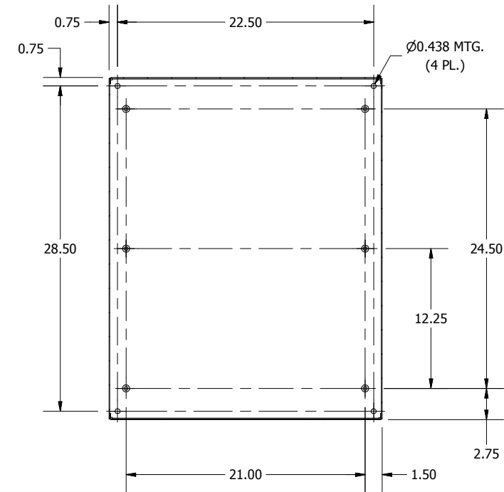
SECTION B-B (INSIDE BACK OF ENCL.)
