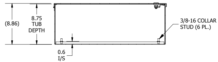
SECTION A-A (INSIDE TOP OF ENCL.)
