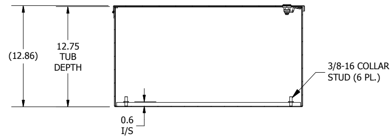
SECTION A-A (INSIDE TOP OF ENCL.)
