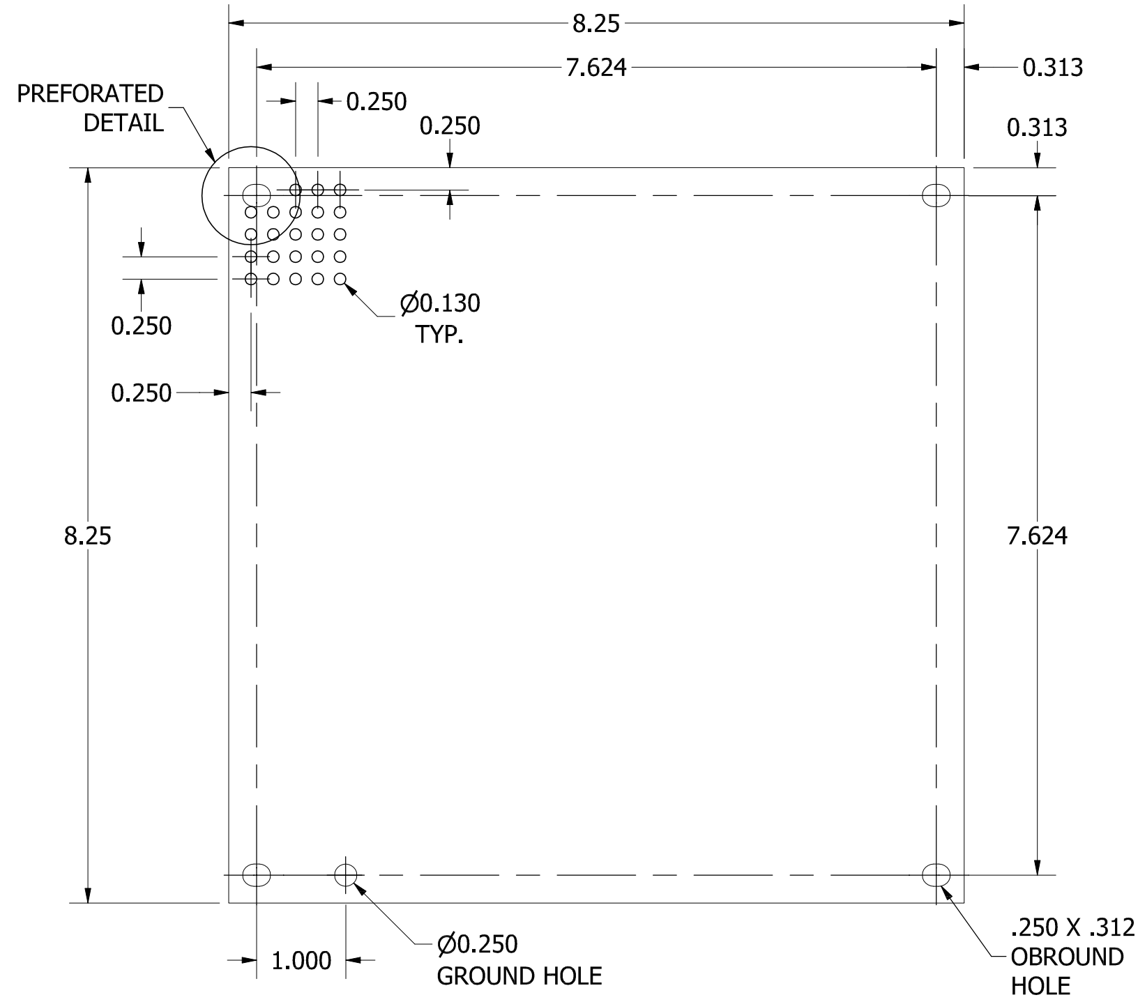
FRONT VIEW
