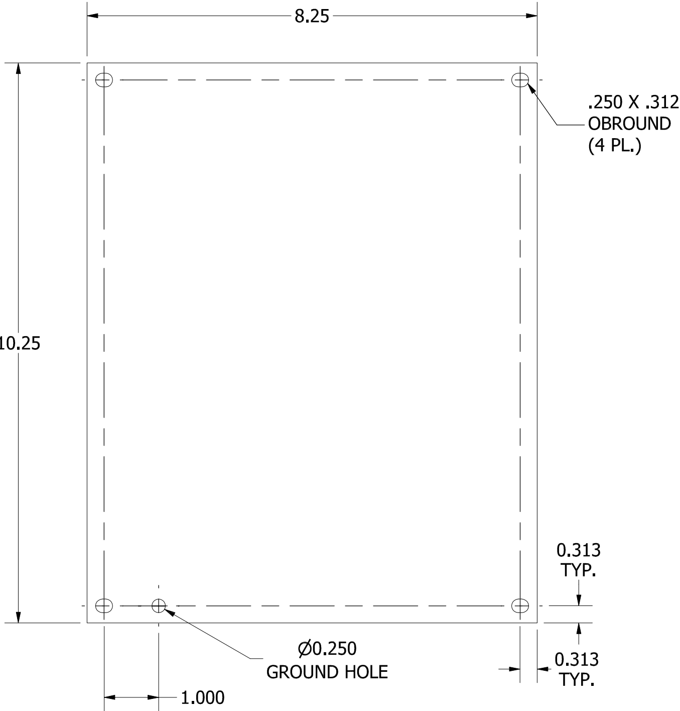
FRONT VIEW
