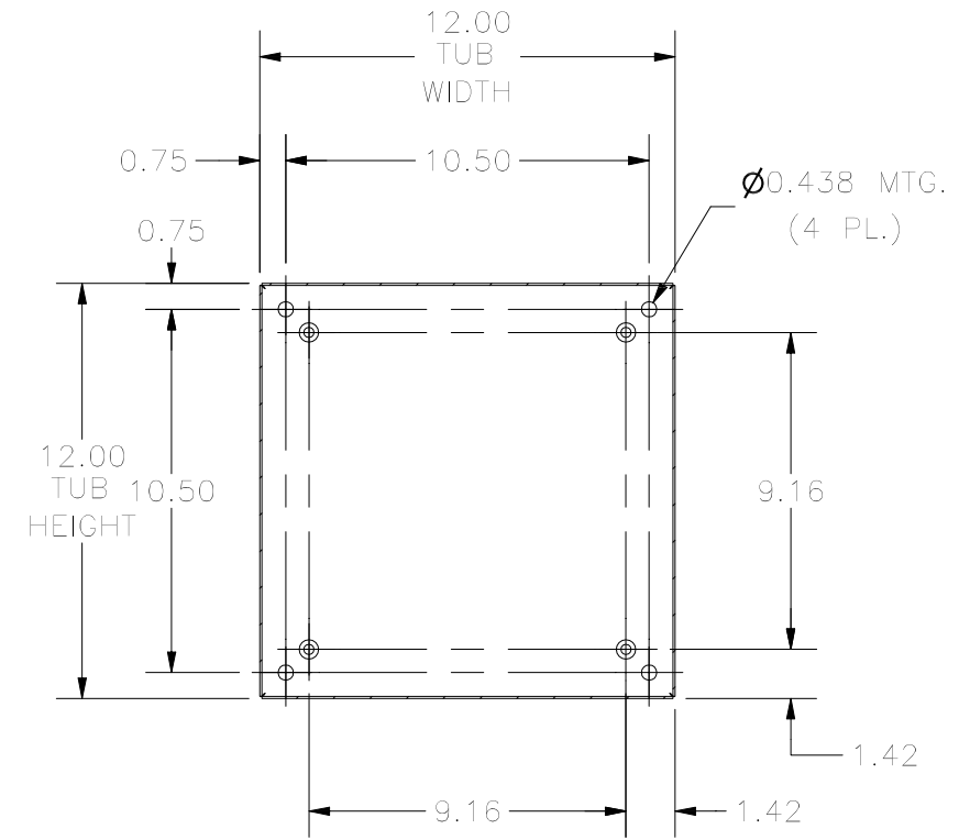
SECTION W-W (INSIDE BACK OF ENCLOSURE)
