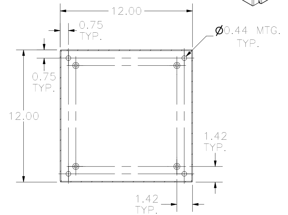
SECTION A-A (INSIDE BACK OF ENCLOSURE)
