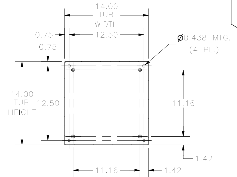
SECTION W-W (INSIDE BACK OF ENCLOSURE)
