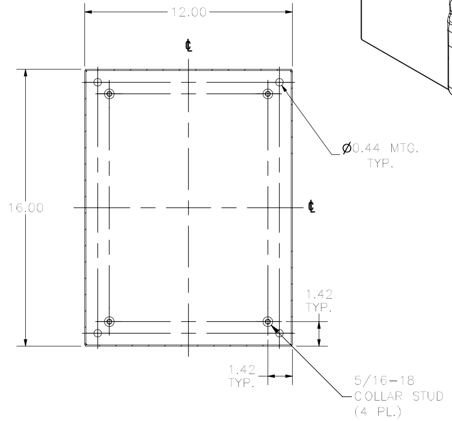
SECTION D-D VIEW (INSIDE BACK OF ENCLOSURE)
