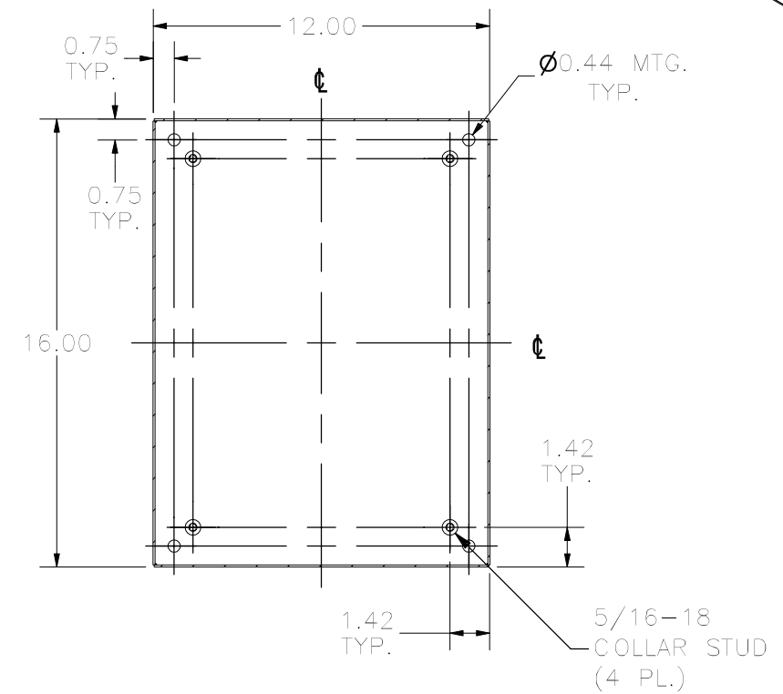
SECTION D-D VIEW (INSIDE BACK OF ENCLOSURE)
