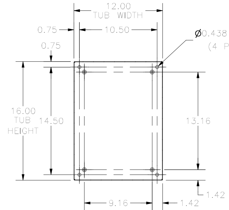
SECTION W-W (INSIDE BACK OF ENCLOSURE)
