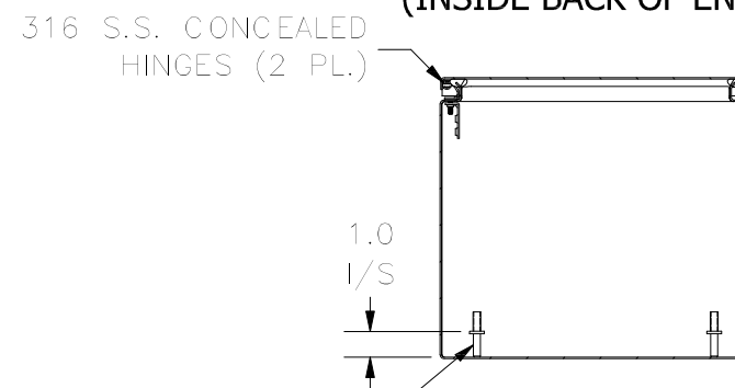
SECTION Y-Y (INSIDE TOP OF ENCLOSURE)
