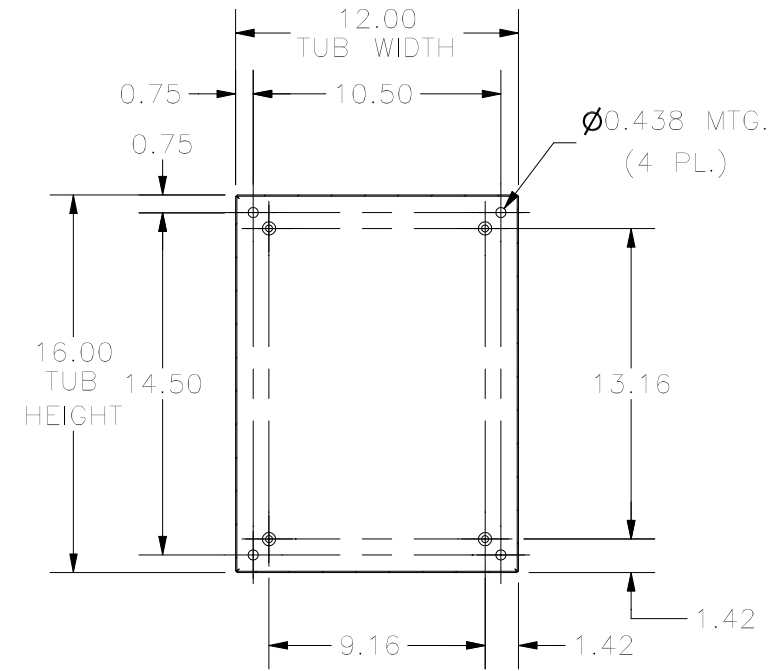
SECTION W-W (INSIDE BACK OF ENCLOSURE)
