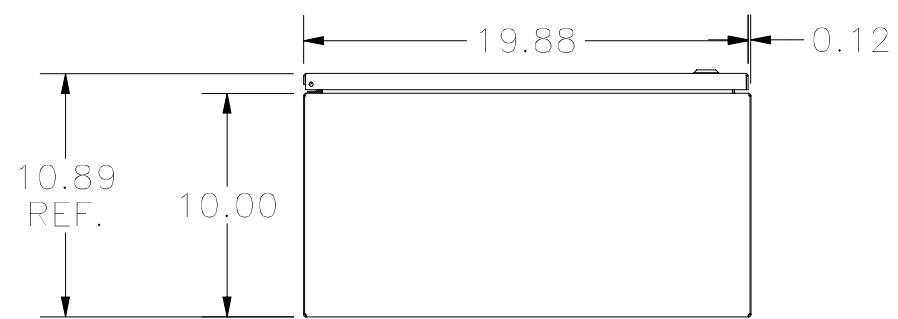
BOTTOM VIEW
