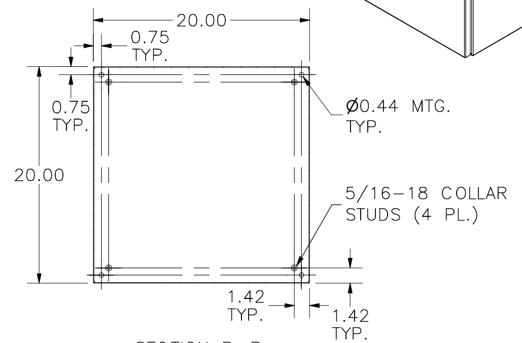
SECTION B-B (INSIDE BACK OF ENCLOSURE)
