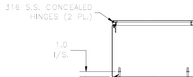
SECTION Y-Y (INSIDE TOP OF ENCLOSURE)
