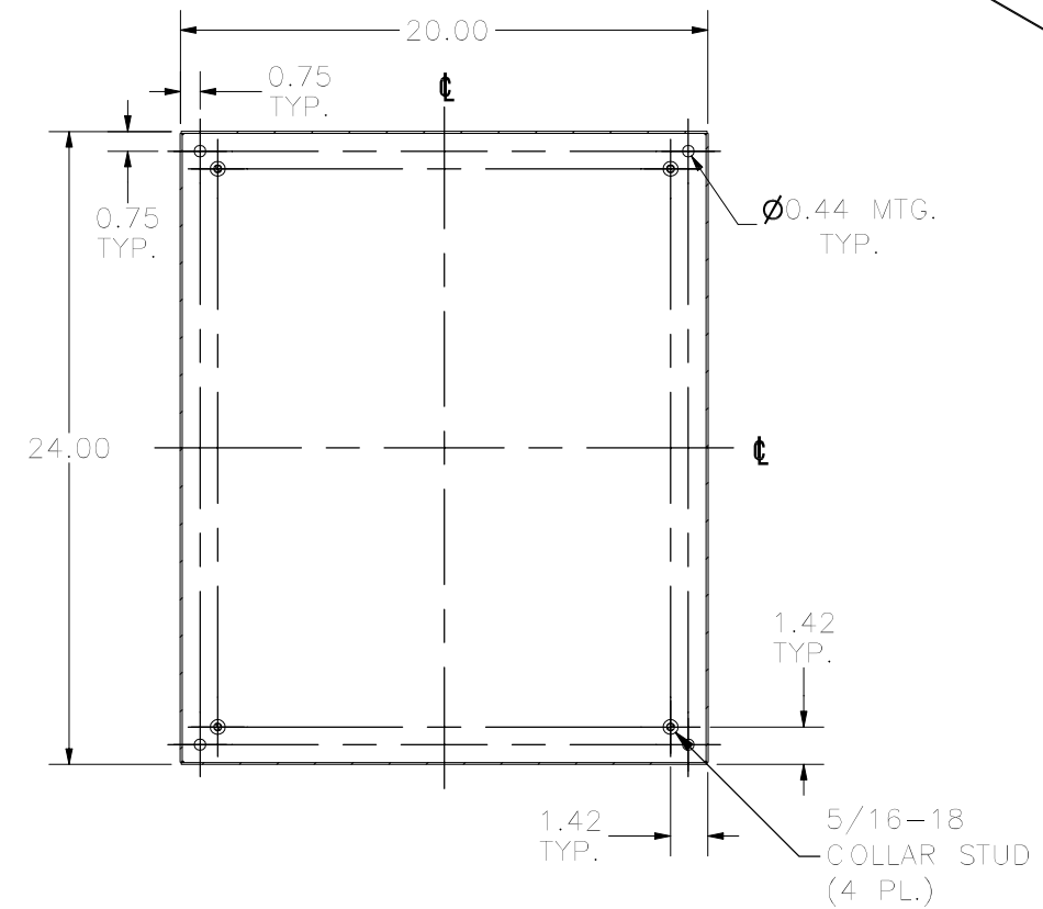
SECTION D-D VIEW (INSIDE BACK OF ENCLOSURE)
