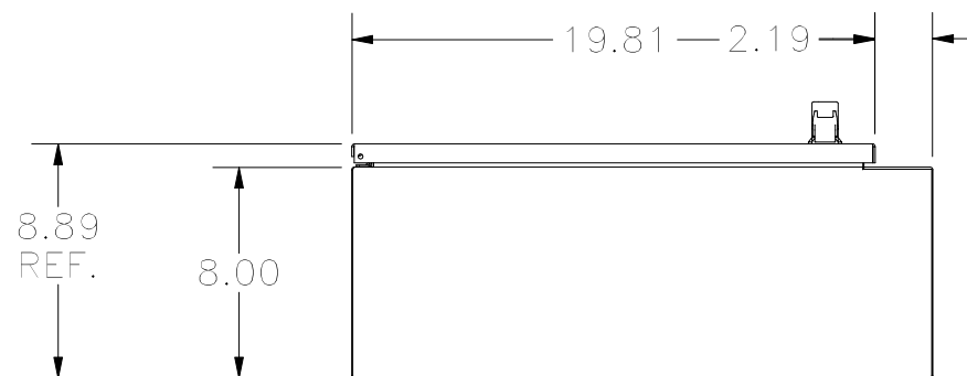
BOTTOM VIEW
