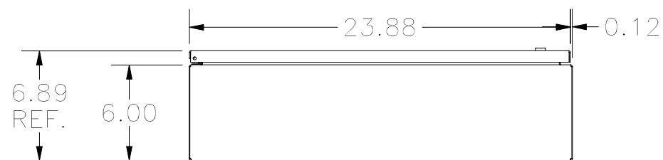
BOTTOM VIEW
