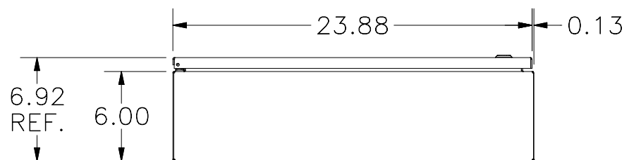
BOTTOM VIEW
