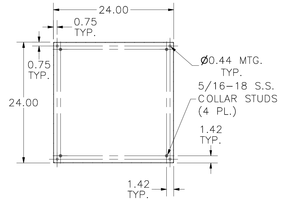
SECTION A-A (INSIDE BACK OF ENCLOSURE)
