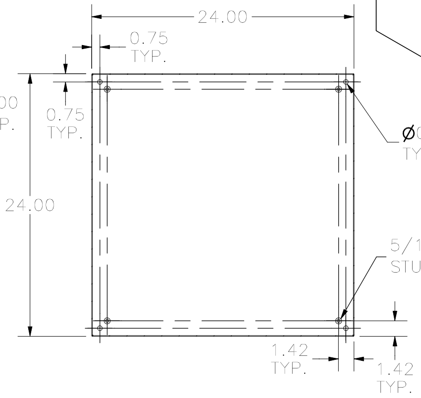
SECTION B-B (INSIDE BACK OF ENCLOSURE)
