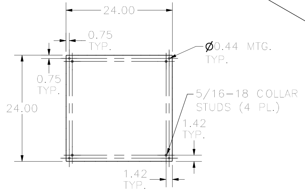
SECTION A-A (INSIDE BACK OF ENCLOSURE)
